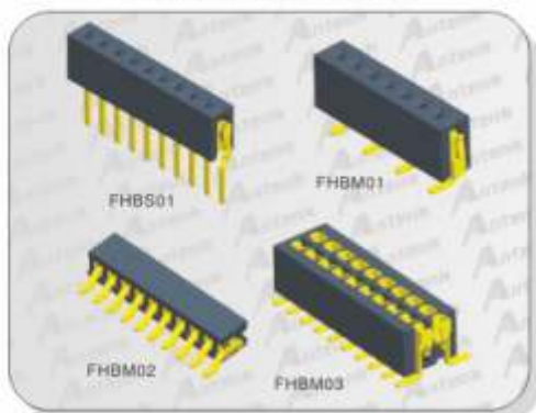
1.27*2.54mm Female Header
