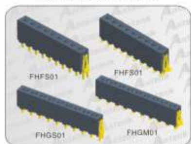
3.96mm Female Header
