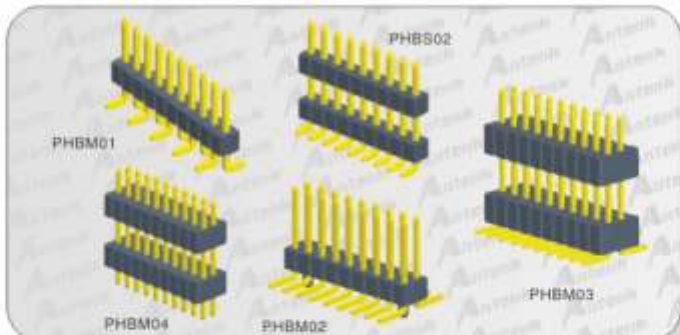
1.27*2.54mm Pin Header
