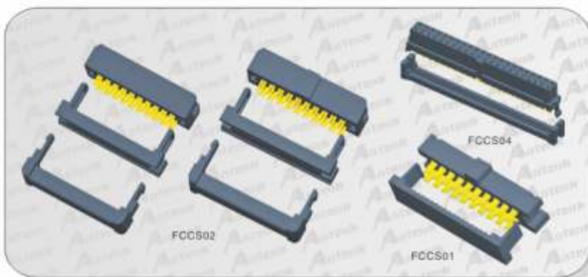
2.00mm IDC Socket Connectors
