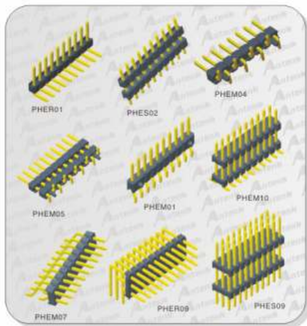
5.08mm Pin Header
